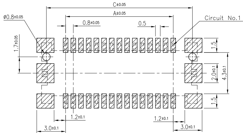
PCB PATTERN LAYOUT
